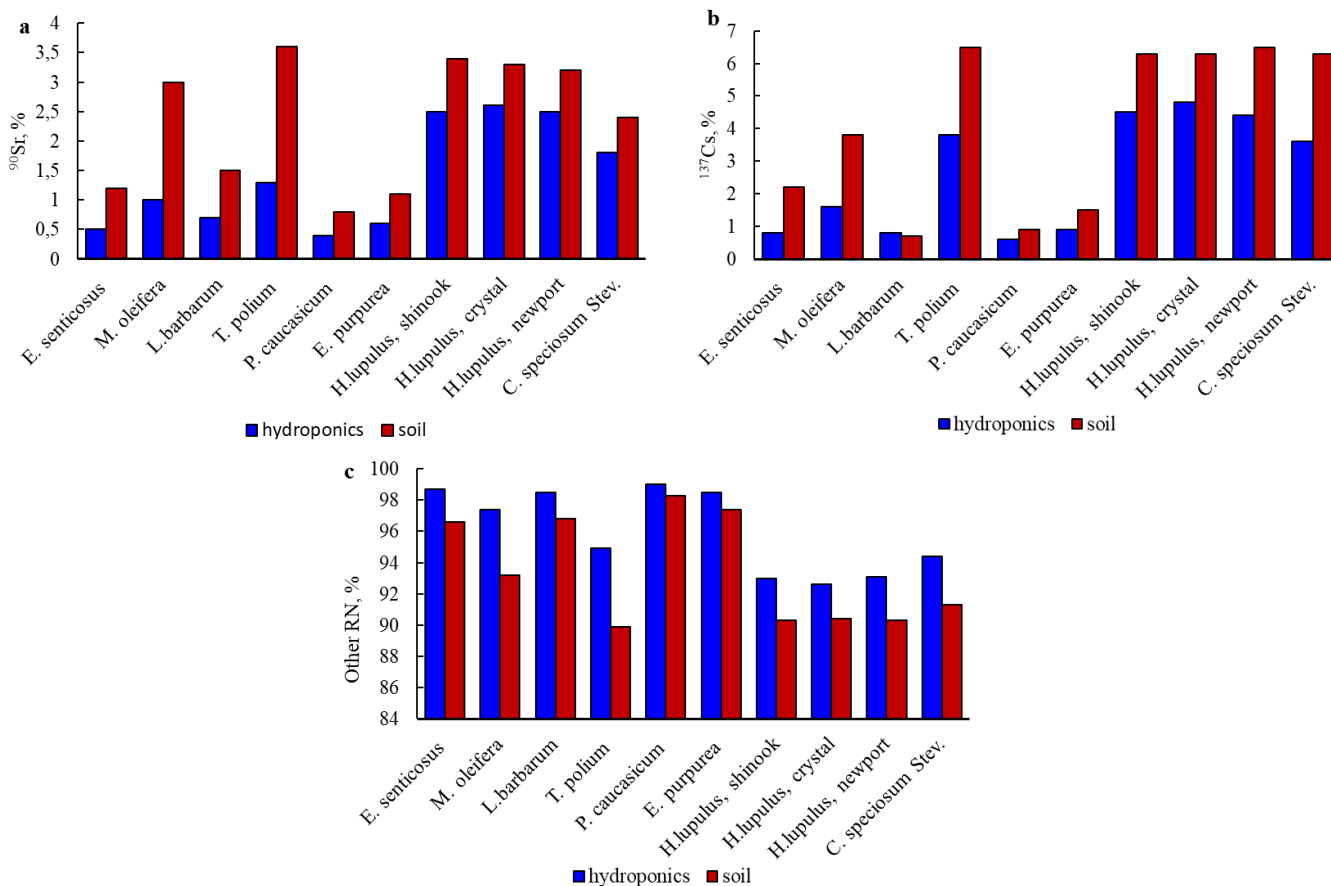
Figure 9: The share of 90 Sr (a), 137 Cs (b), and other RN (except 90 Sr, 137 Cs) (c) in gross β-radioactivity in medicinal plants in hydroponics and soil
