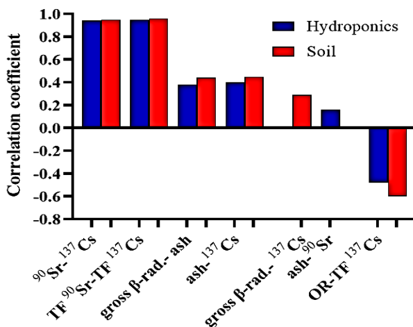
Figure 11: Correlation coefficients between agro-radiochemical indices of medicinal plant in hydroponics and soil. The correlation between the pairs ( 90 Sr - 137 Cs couple, TF 90 Sr - TF 137 Cs couple) is significant, since t_{actual} > t_{theoretical} , t_{05} = 2,23 .
