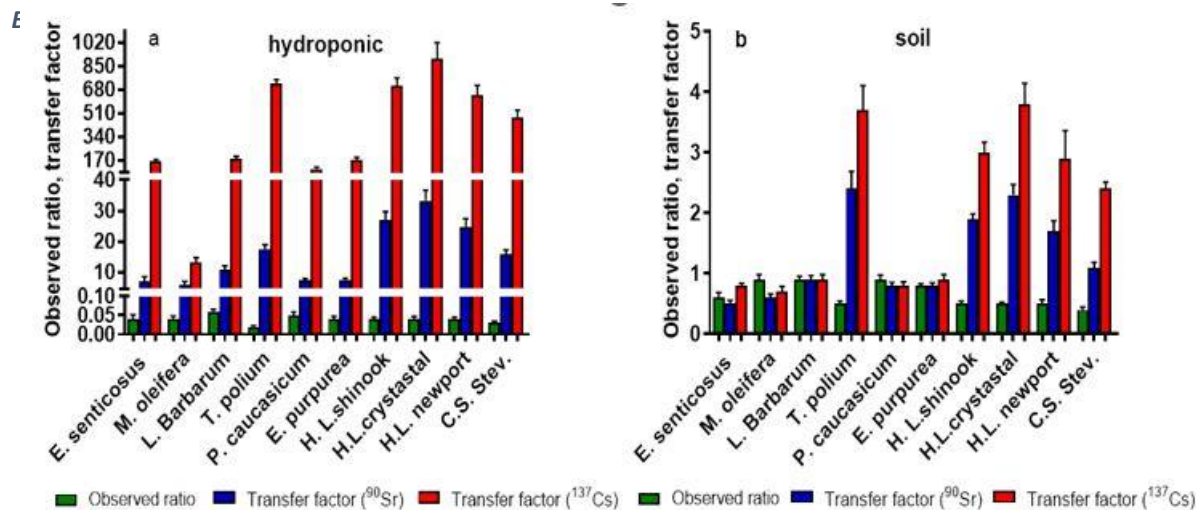
Figure 10: Observed ratio and transfer factor of 90 Sr - 137 Cs couple in nutrient solution - plant (a) and soil - plant (b) systems for s medicinal plants
