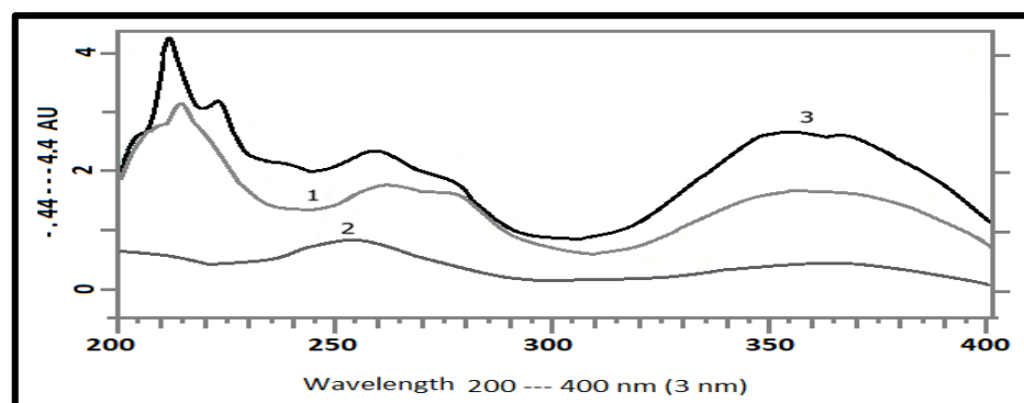
Figure 2. The ultraviolet (UV)-spectrum of fractions (1 – quercetagenin di-glycosides, 2 – quercetin di-glycosides, 3 – quercetin and quercetin glycosides) extracted from French Marigold ( Tagetes patula L.) (quercetin-rich flavonoid fraction is shown in blue)
