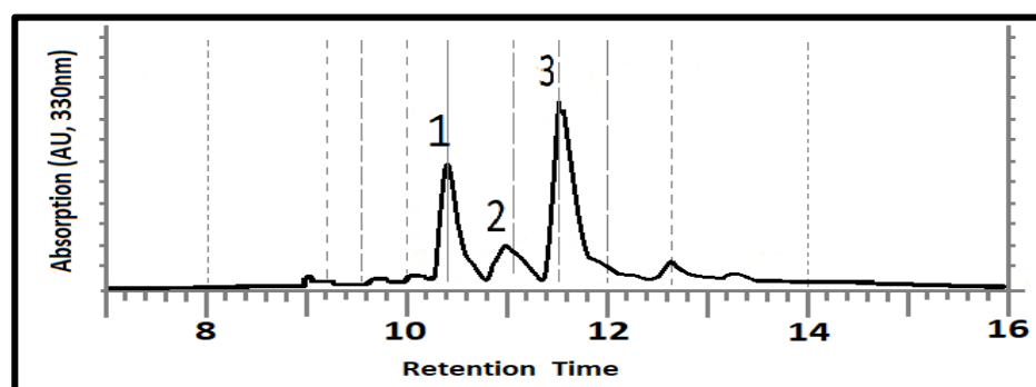
Figure 1. HPLC chromatograms of three main fractions (1 – quercetagenin diglycosides, 2 – quercetin diglycosides, 3 – quercetin and quercetin glycosides) extracted from French Marigold ( Tagetes patula L.)
