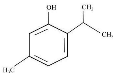
Figure 1. Thymol structure
