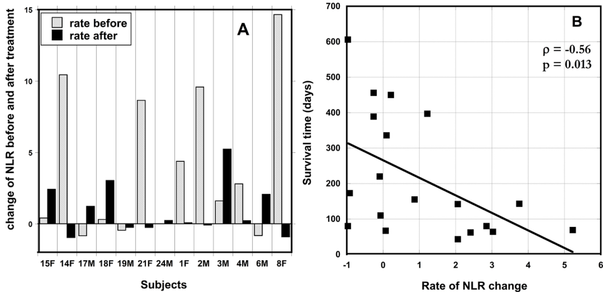
Figure 4. (A) \Delta NLR values pre-IVC and at the end IVC therapy (post). (B) Correlation between patient survival time (days after start of therapy) and the \Delta NLR value at the end of therapy.
